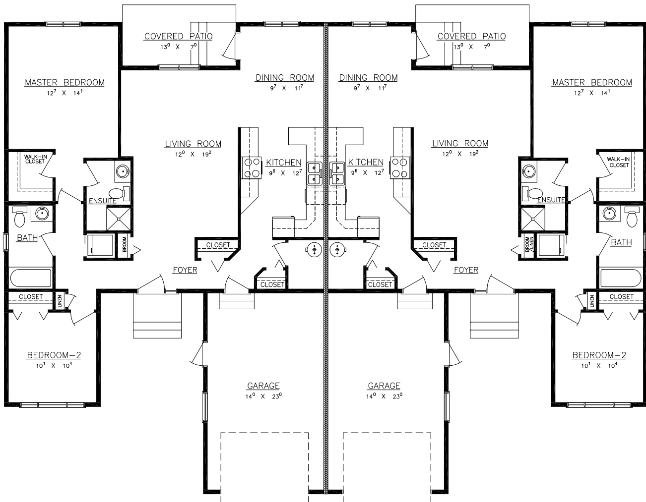
FLOOR PLAN
